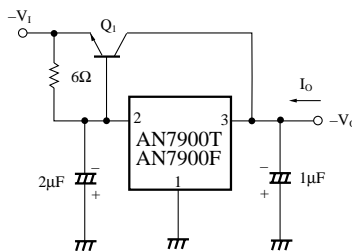
1) Current Bootstrap Circuit
